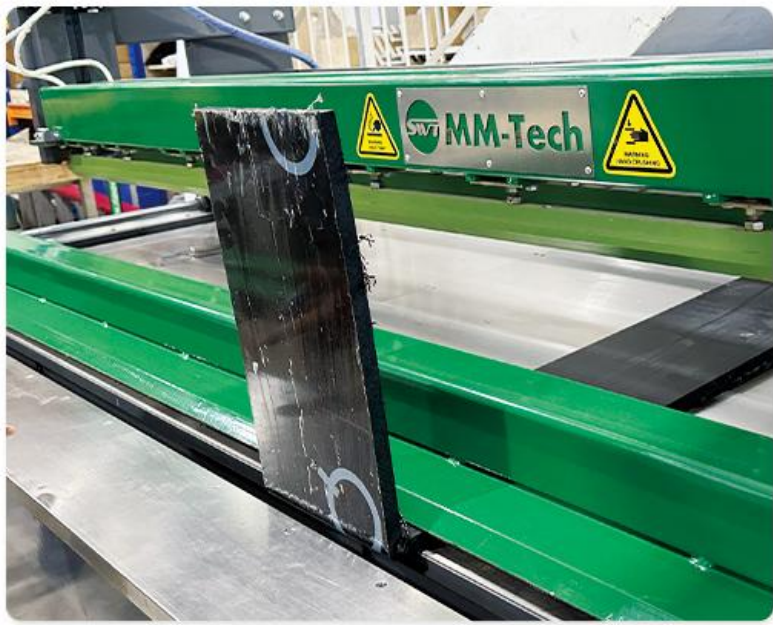
0 - 95° Bending by one sheet
